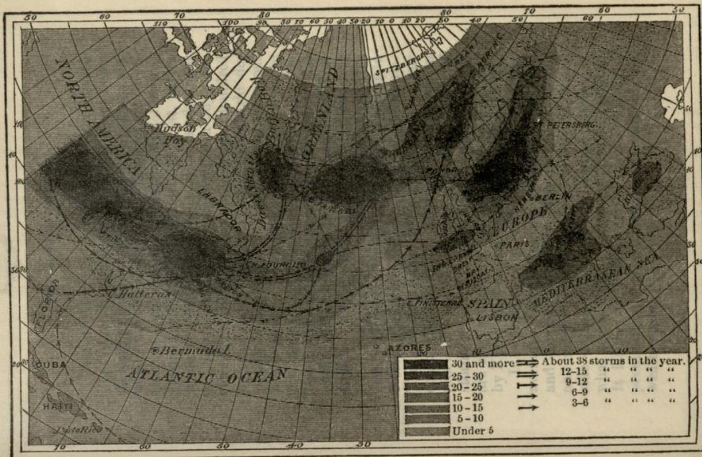
AVERAGE TRACKS OF STORMS FROM THE ROCKY MOUNTAINS TO THE URAL.
